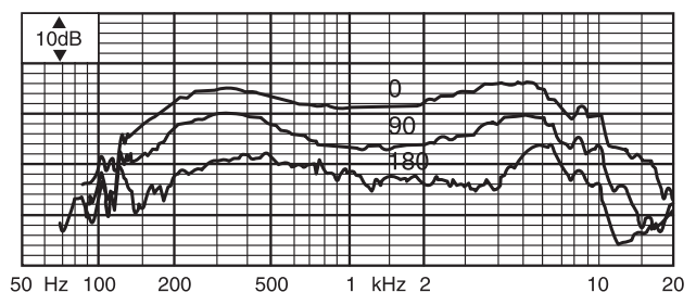
Frequency response
